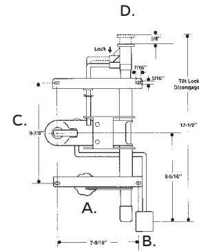
Typical Knee Tilt Control
